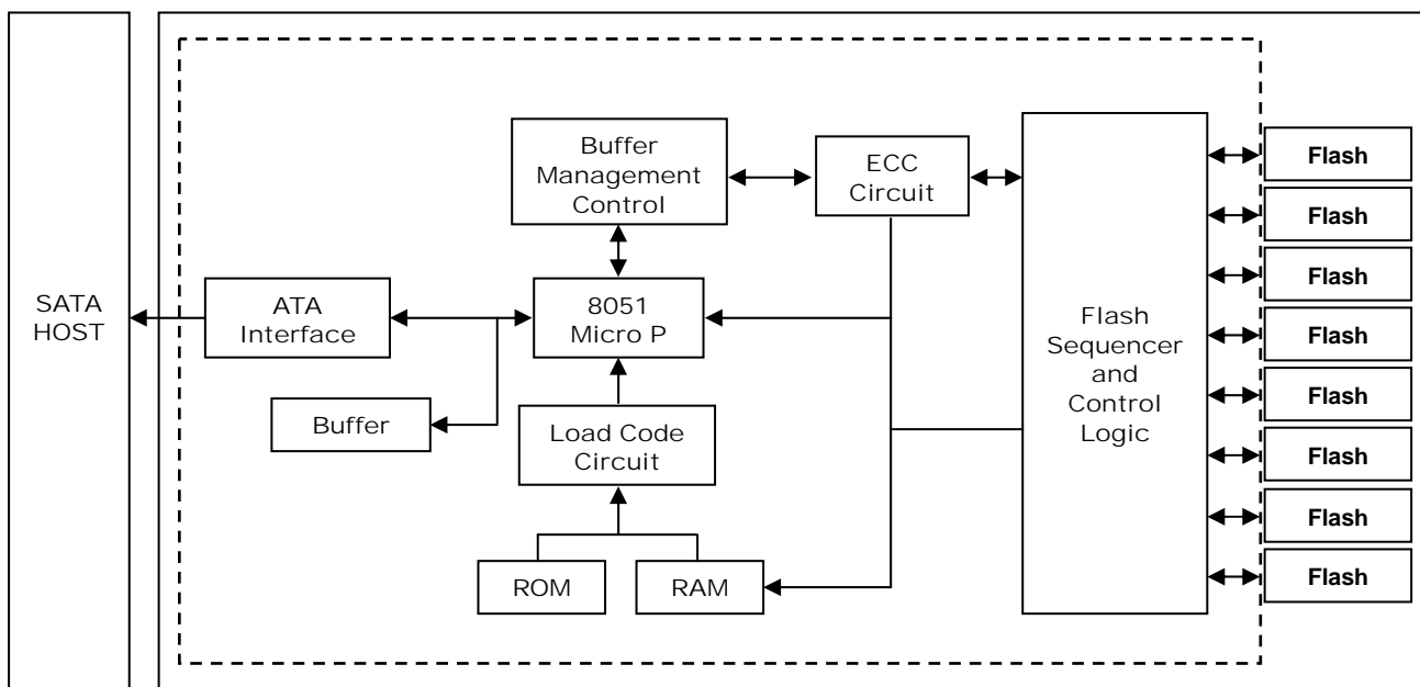
Figure 1: Industrial 1.8" SATA II SLC SSD HERMES Series controller block diagram
