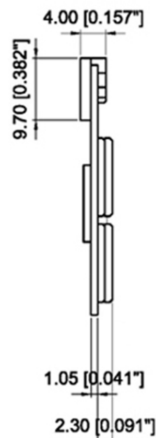
Right Side
