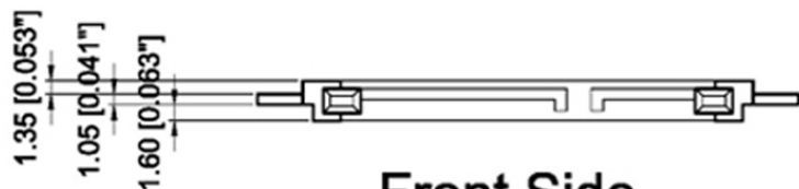
Front Side
