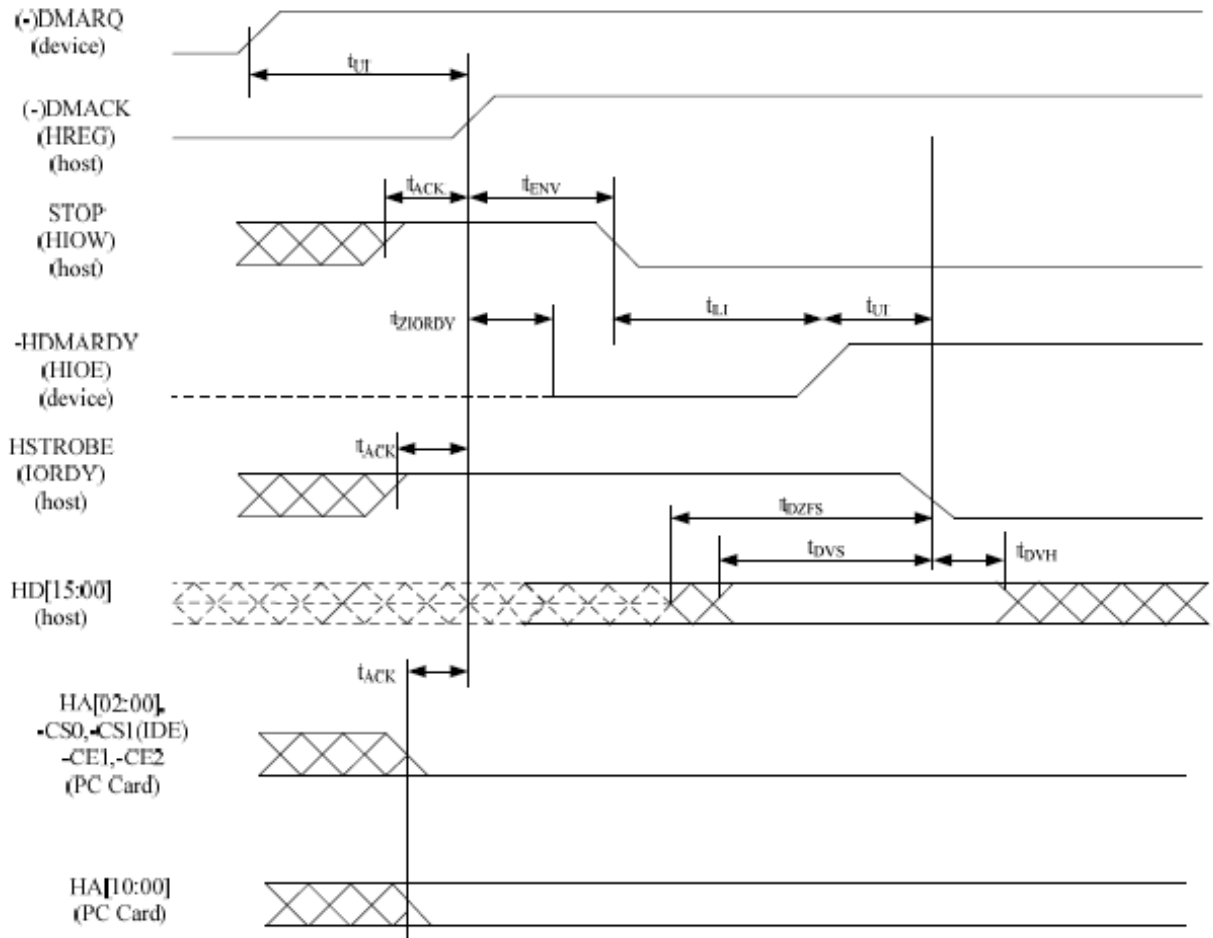
Figure 19: Ultra DMA Data-Out Burst Initiation Timing Diagram
