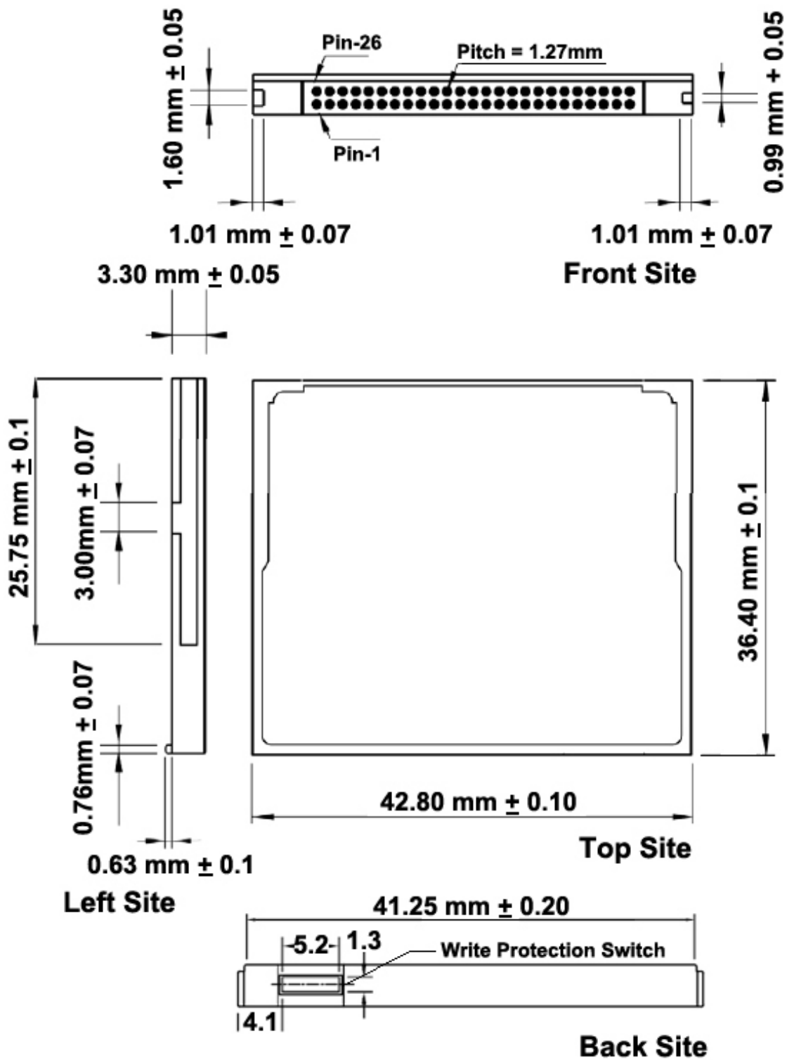
Figure 3: Industrial Write-protect CompactFlash Card Dimension
