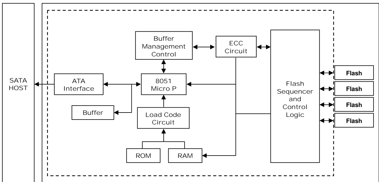
Figure 1: 1.8" Slim Lite SATA II MLC SSD HERMES-D Series controller block diagram
