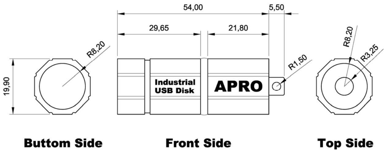
Figure 3: Generation 2 Dimensions
